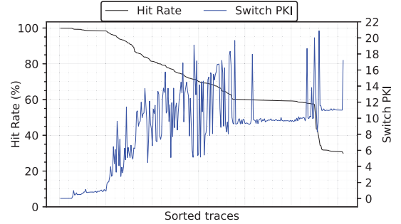
Fig. 3: \mu -op cache hit rate and switch PKI across the CVP-1 traces. Sorted by hit rate.
