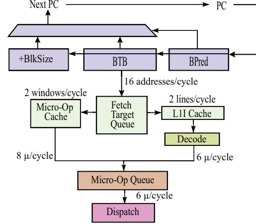
Fig. 1: Processor frontend
