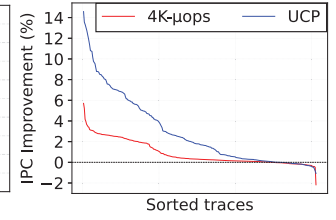
Fig. 10: IPC of UCP and baseline relative to no \mu -op cache
